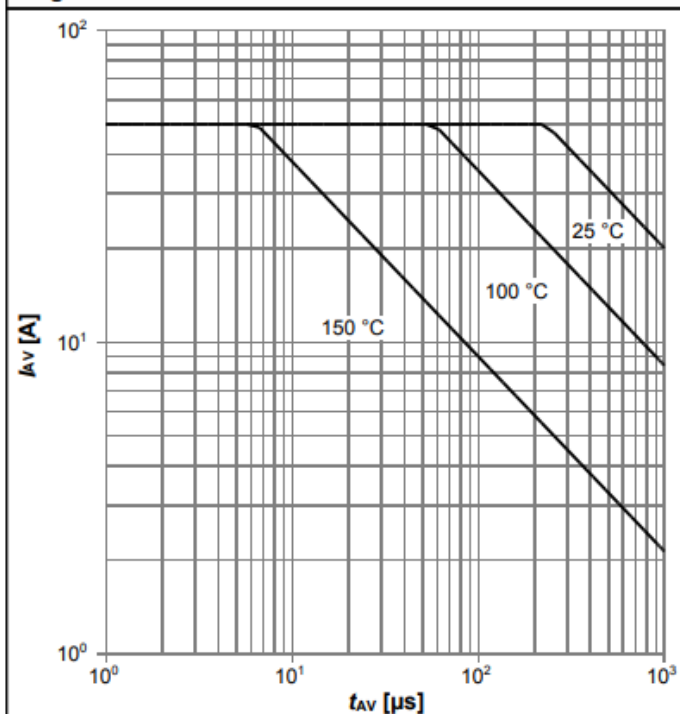
Diagram 13: Avalanche characteristics
