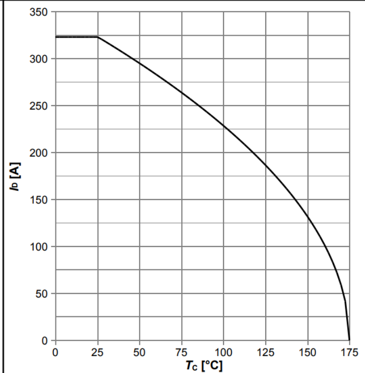
Diagram 2: Drain current
