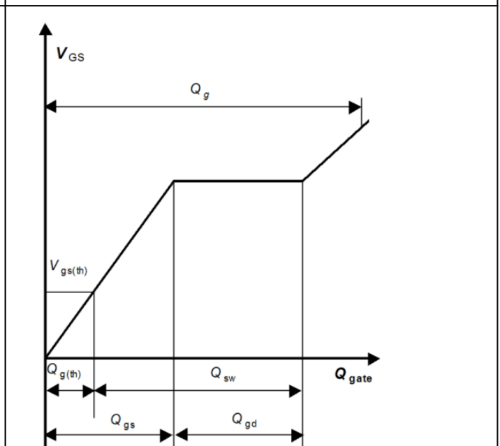
Gate charge waveforms
