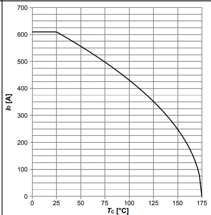
Diagram 2: Drain current
