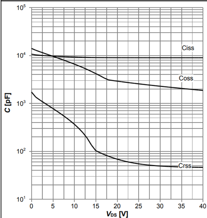
Diagram 11: Typ. capacitances
