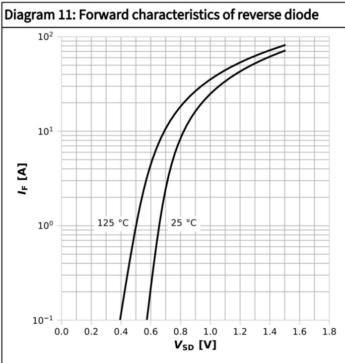
I_F = f(V_{SD}) ; parameter: T_j
