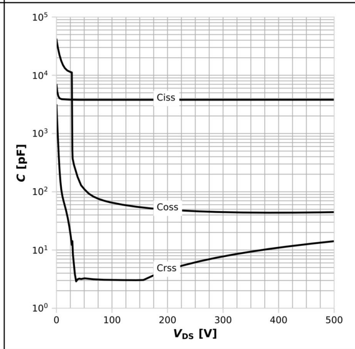
Diagram 14: Typ. capacitances
