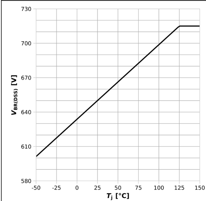
Diagram 13: Drain-source breakdown voltage
