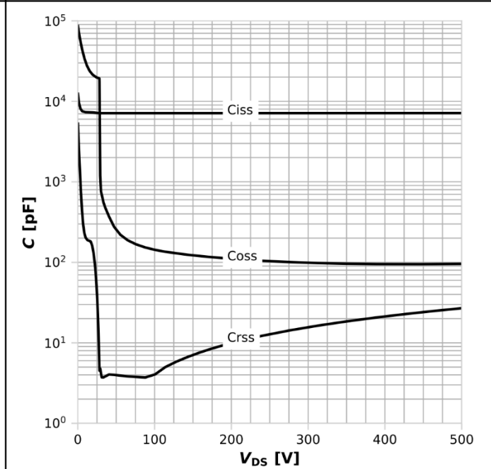
Diagram 14: Typ. capacitances
