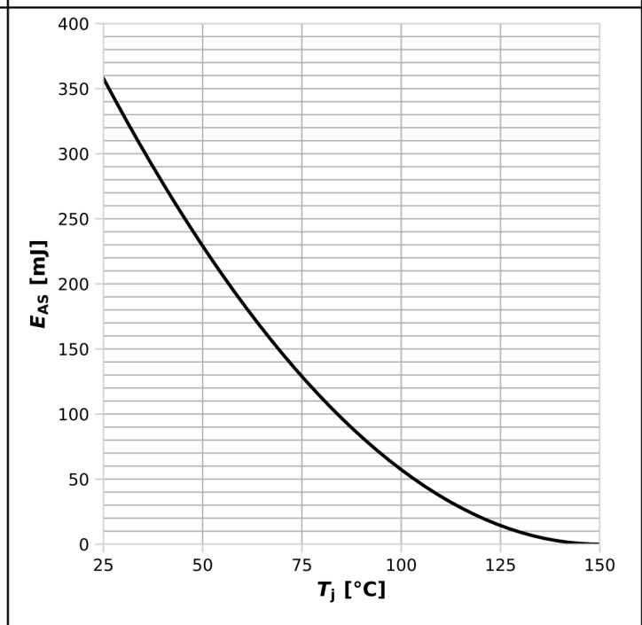
Diagram 12: Avalanche energy
