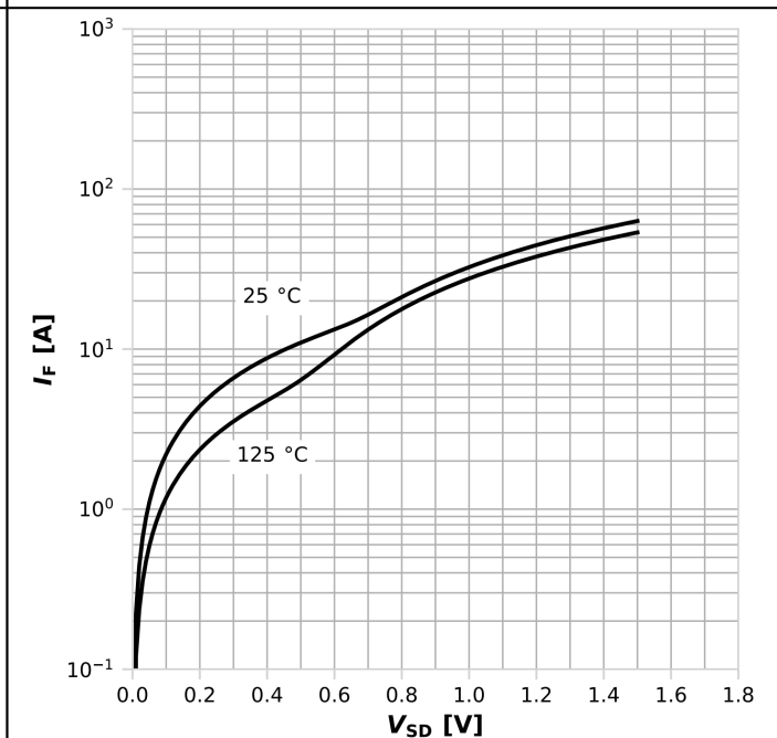
Diagram 16: Forward characteristics of reverse diode
