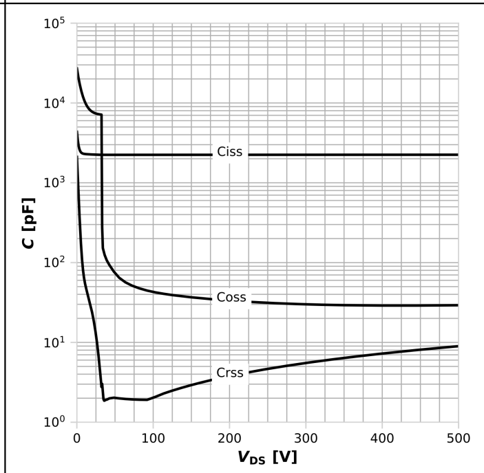
Diagram 14: Typ. capacitances
