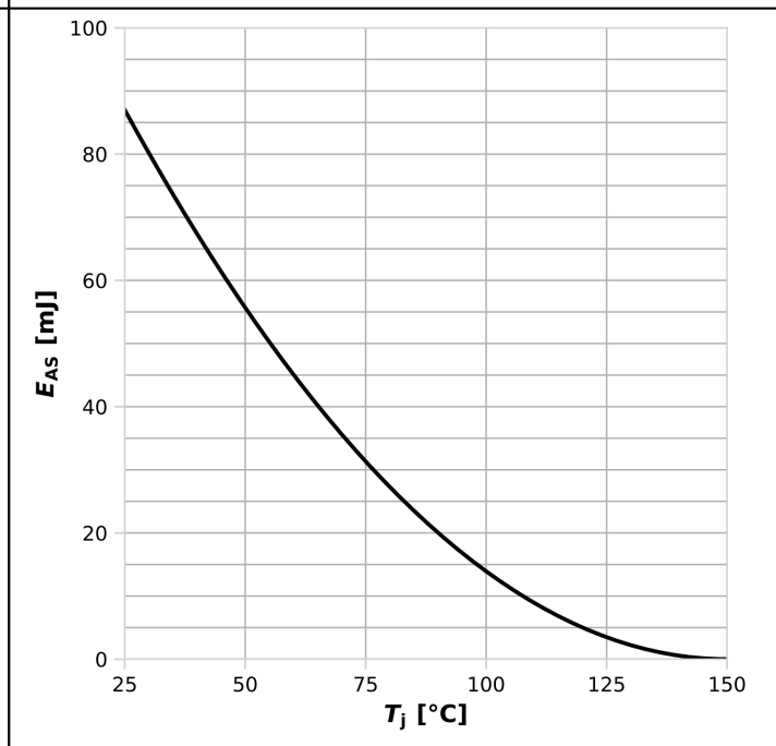
Diagram 12: Avalanche energy
