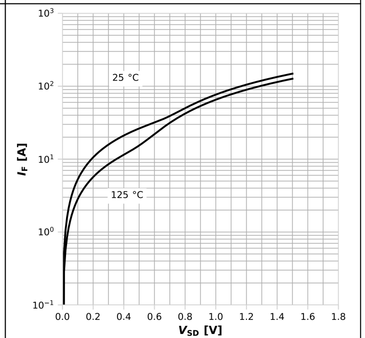
Diagram 16: Forward characteristics of reverse diode
