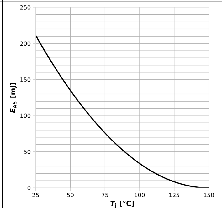
Diagram 12: Avalanche energy
