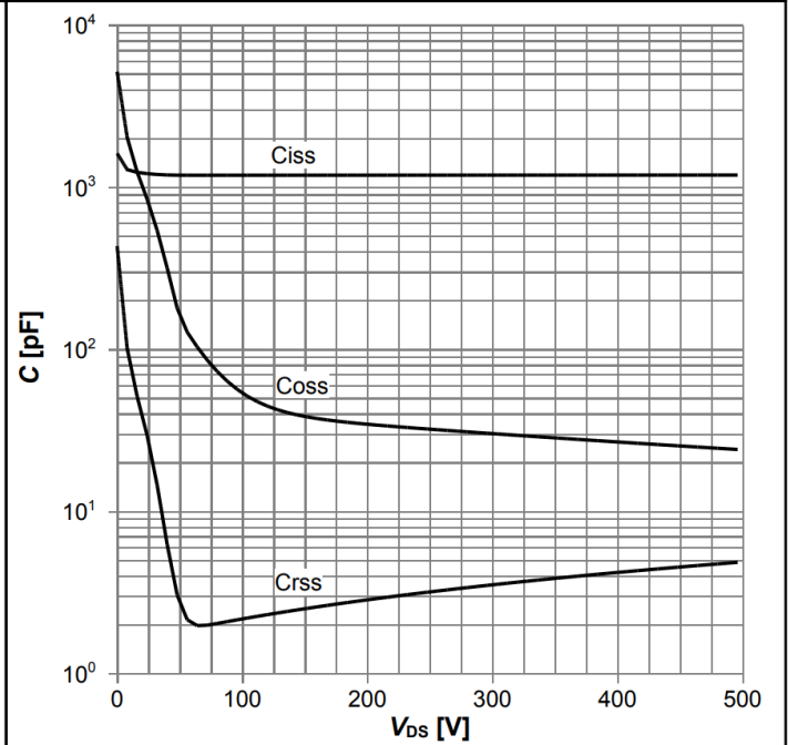
Diagram 18: Typ. capacitances
