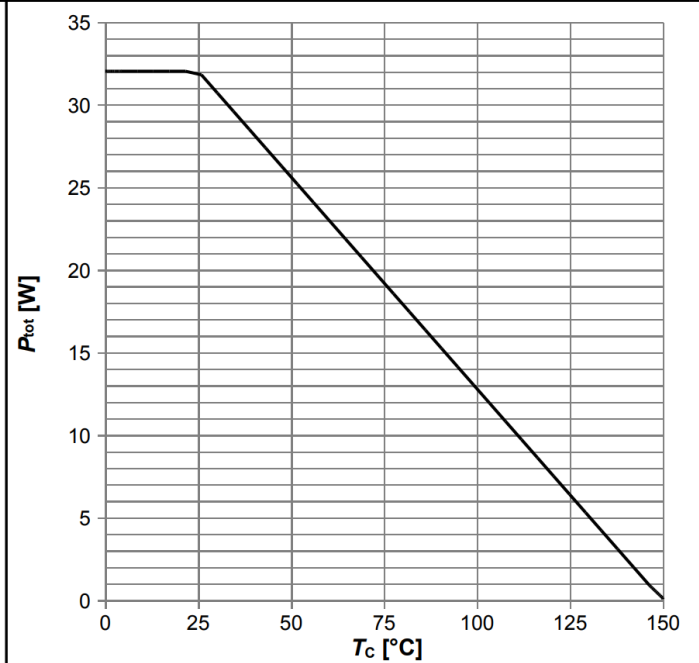
Diagram 2: Power dissipation (FullPAK)
