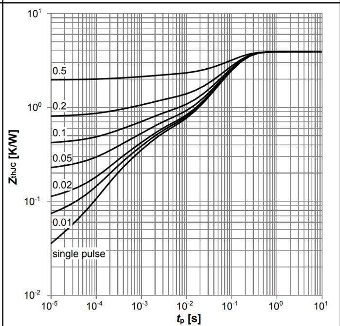
Diagram 4: Max. transient thermal impedance (FullPAK)
