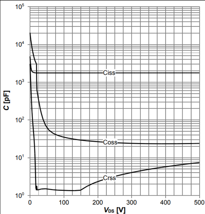
Diagram 14: Typ. capacitances
