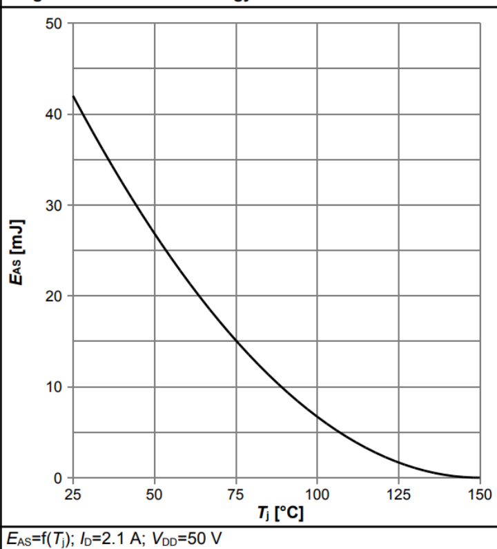
Diagram 12: Avalanche energy
