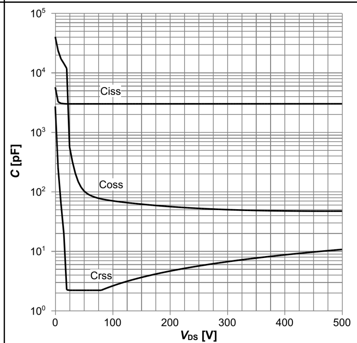
Diagram 14: Typ. capacitances
