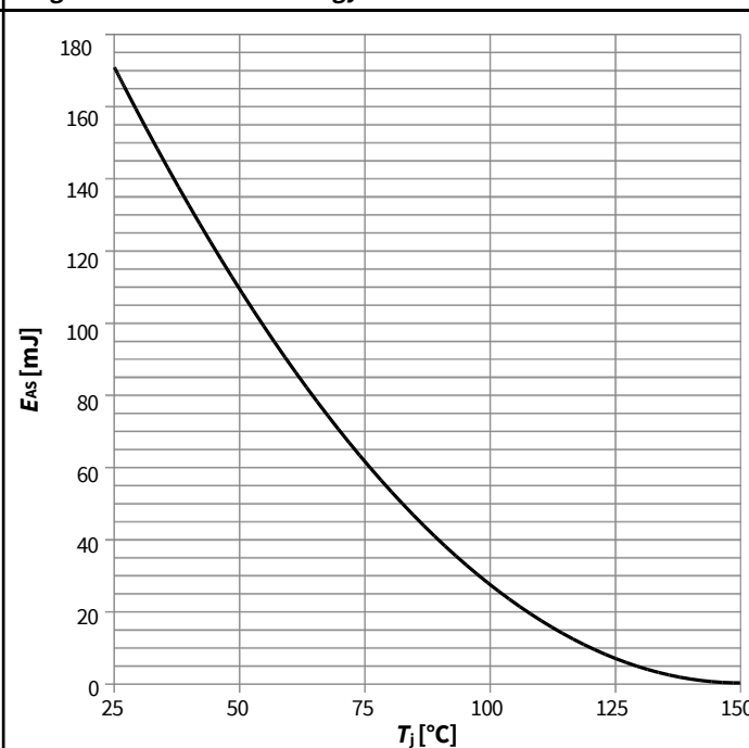
Diagram 12: Avalanche energy
