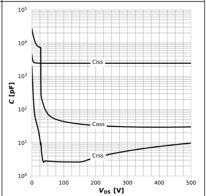
Diagram 14: Typ. capacitances
