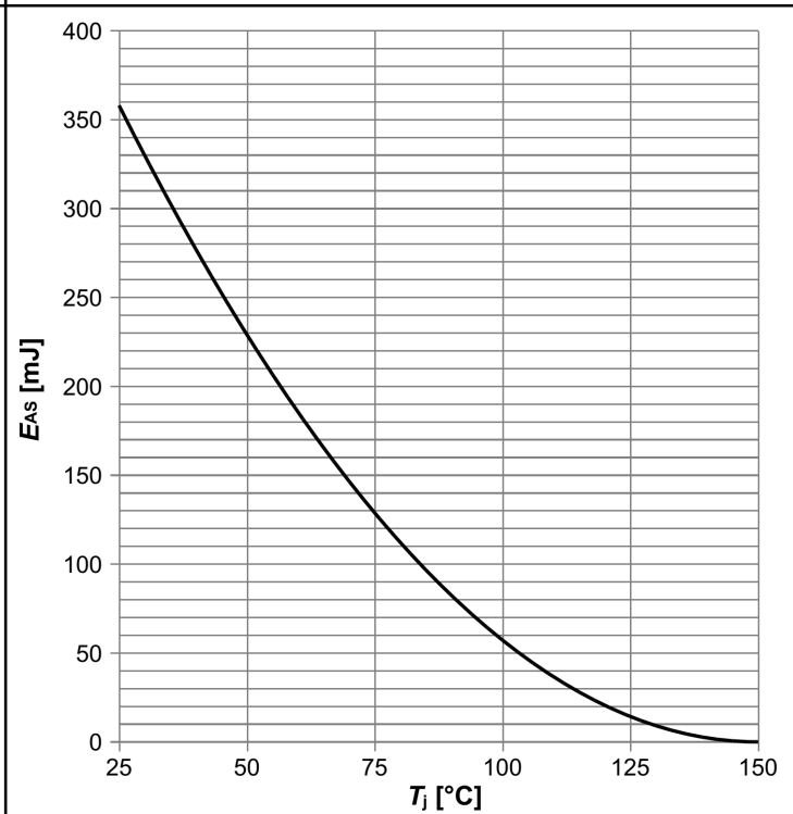
Diagram 12: Avalanche energy
