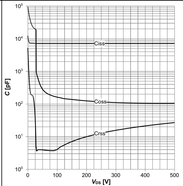
Diagram 14: Typ. capacitances
