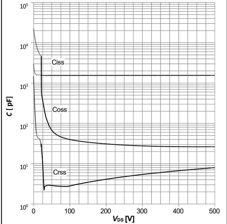
Diagram 14: Typ. capacitances
