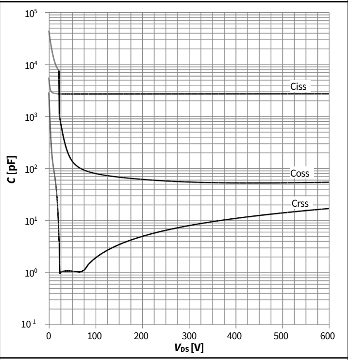
Diagram 14: Typ. capacitances
