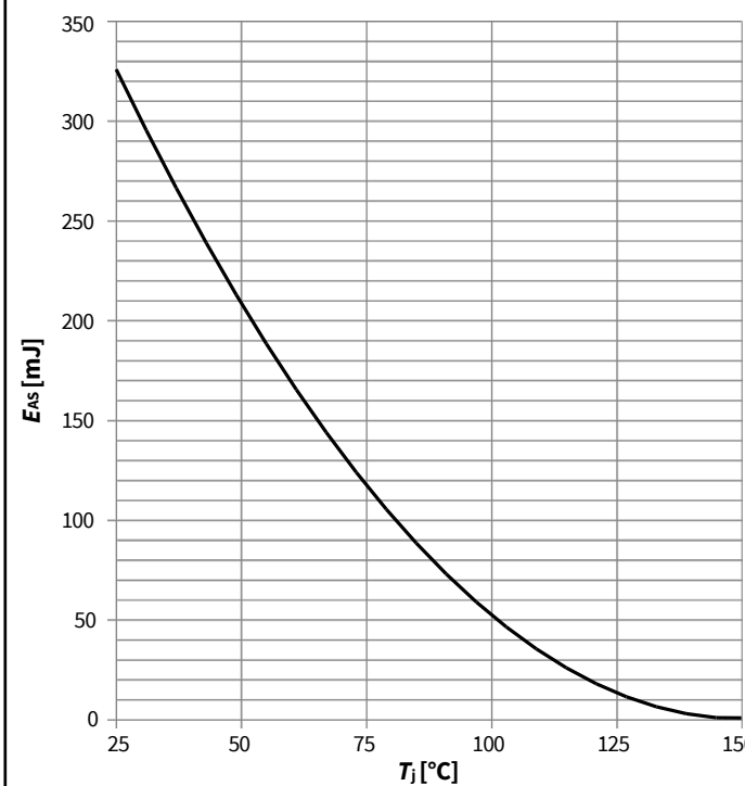
Diagram 12: Avalanche energy
