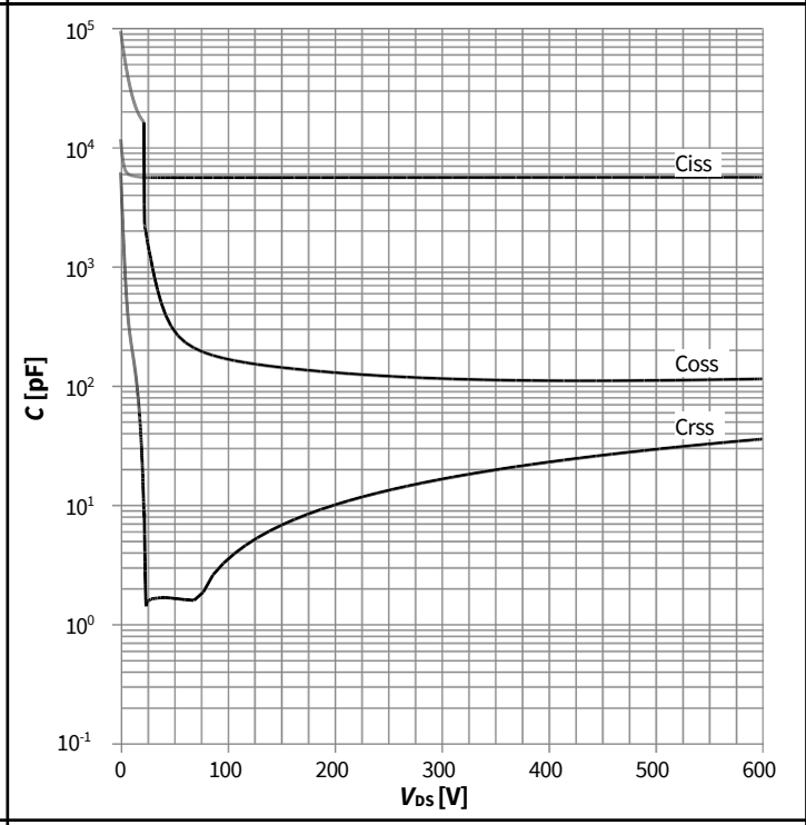
Diagram 14: Typ. capacitances
