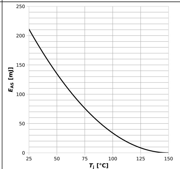
Diagram 12: Avalanche energy
