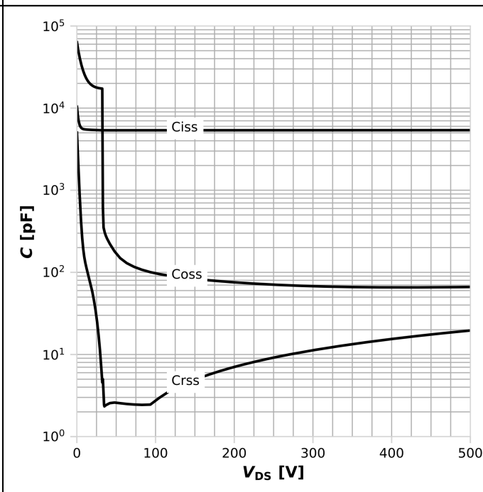
Diagram 14: Typ. capacitances
