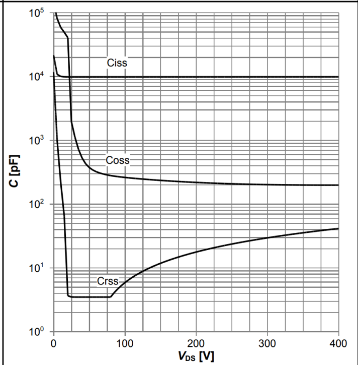
Diagram 14: Typ. capacitances
