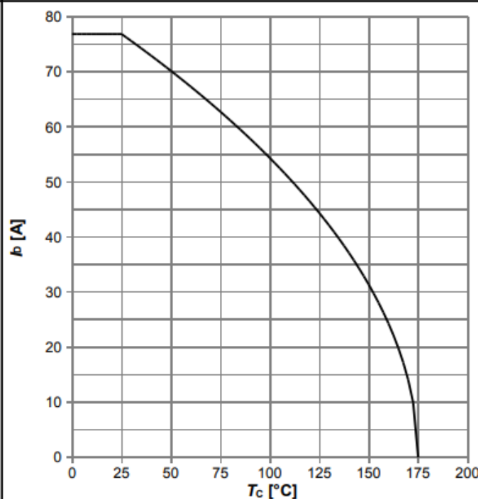
Diagram 2: Drain current
