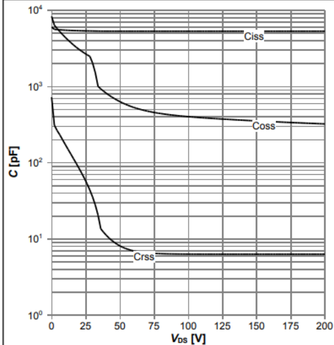
Diagram 11: Typ. capacitances
