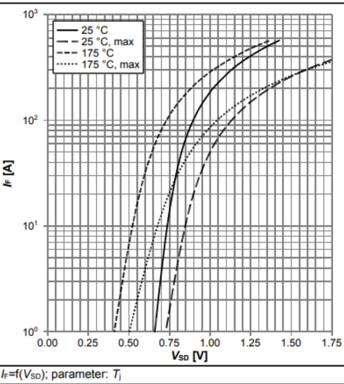
Diagram 12: Forward characteristics of reverse diode
