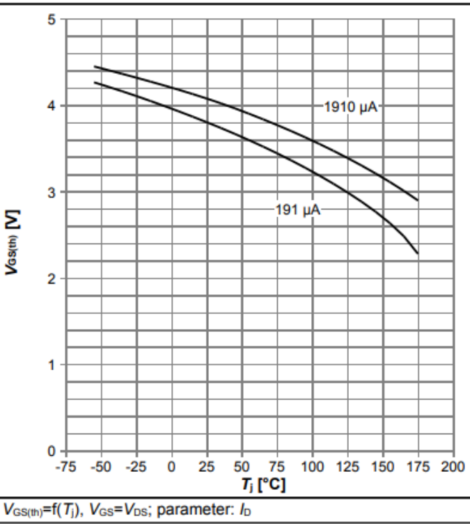
Diagram 10: Typ. gate threshold voltage
