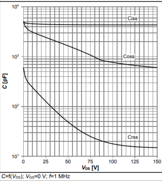
Diagram 11: Typ. capacitances
