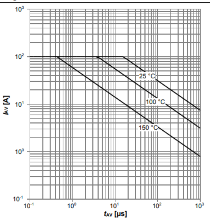
Diagram 13: Avalanche characteristics
