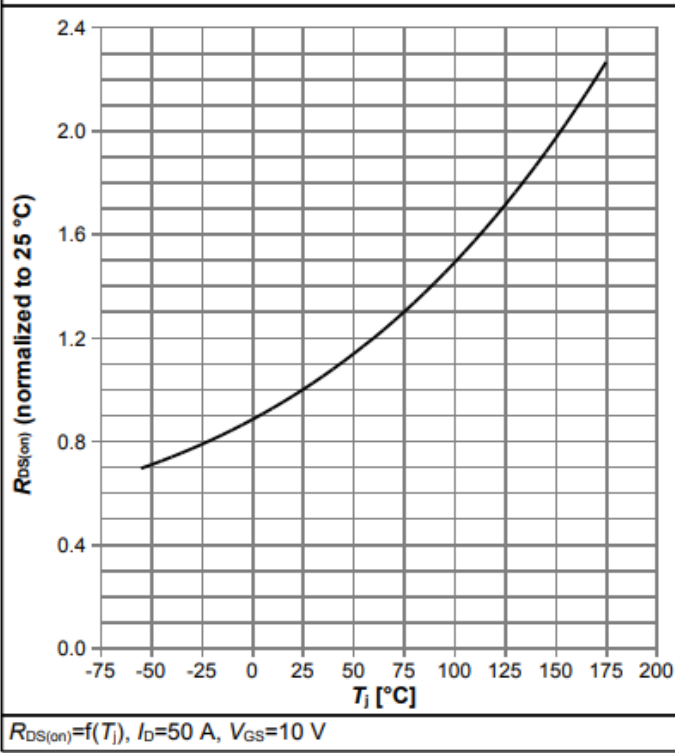
Diagram 9: Normalized drain-source on resistance
