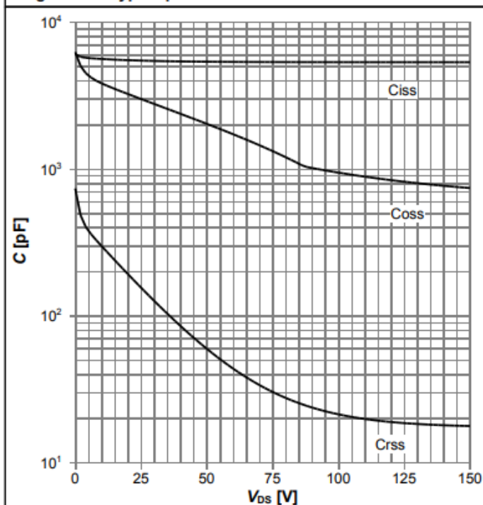
Diagram 11: Typ. capacitances
