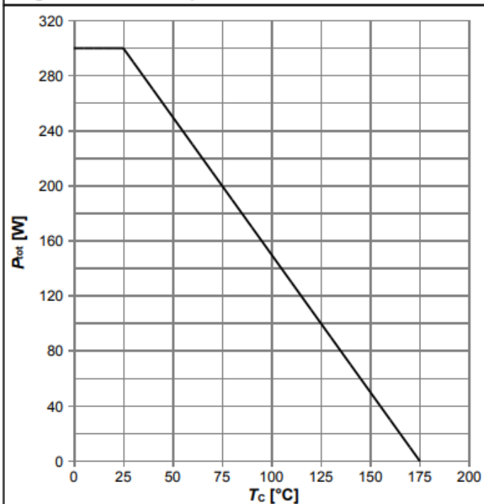
Diagram 1: Power dissipation
