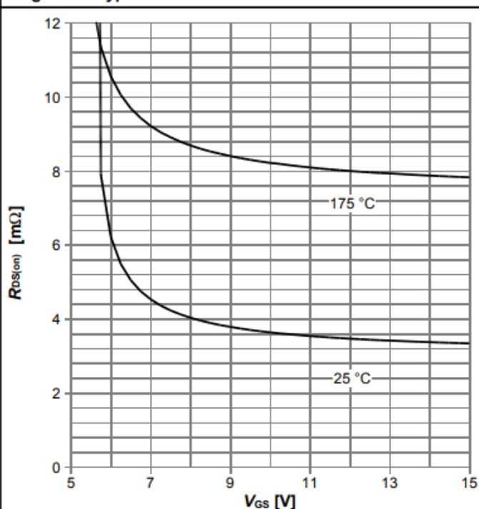
Diagram 8: Typ. drain-source on resistance
