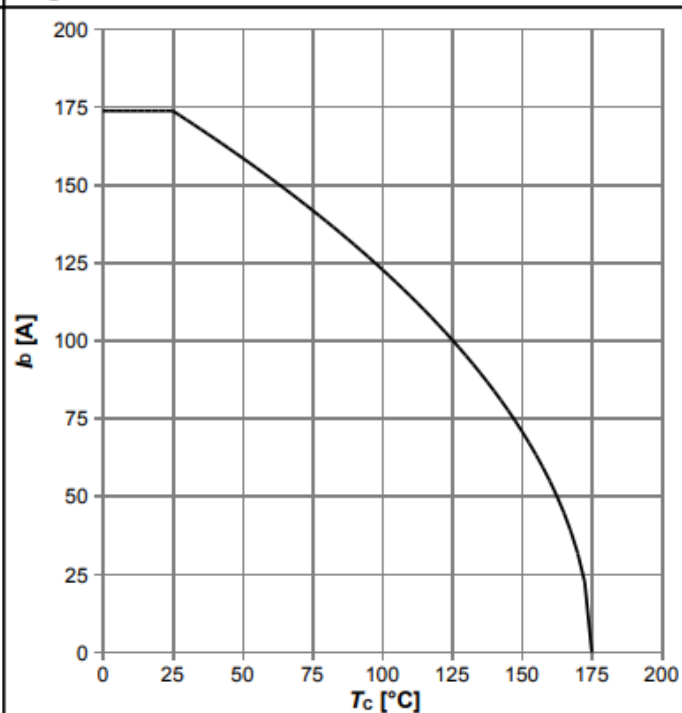
Diagram 2: Drain current
