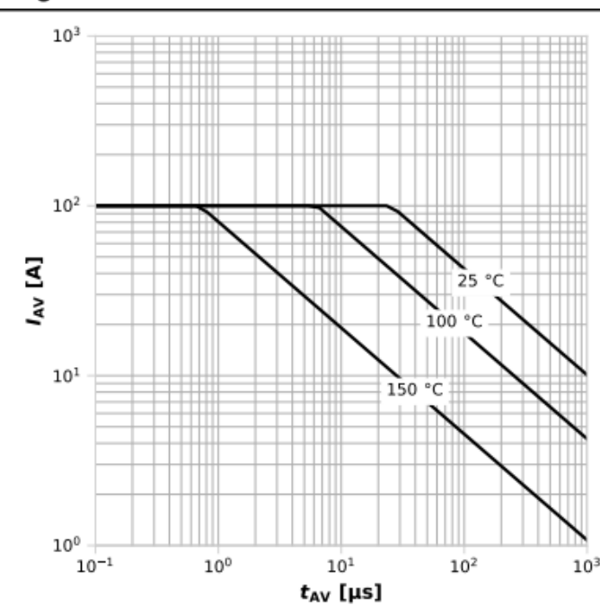
Diagram 13: Avalanche characteristics
