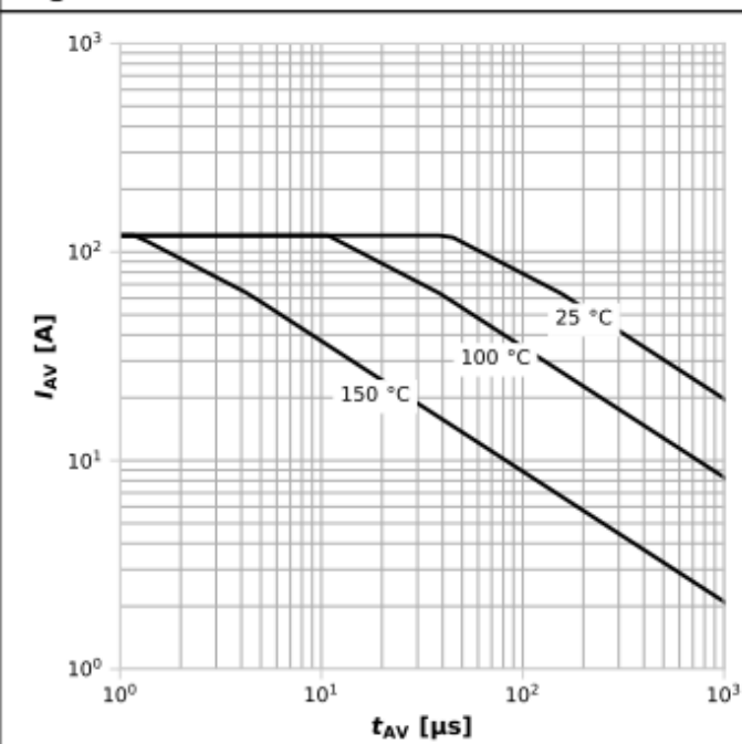
Diagram 13: Avalanche characteristics
