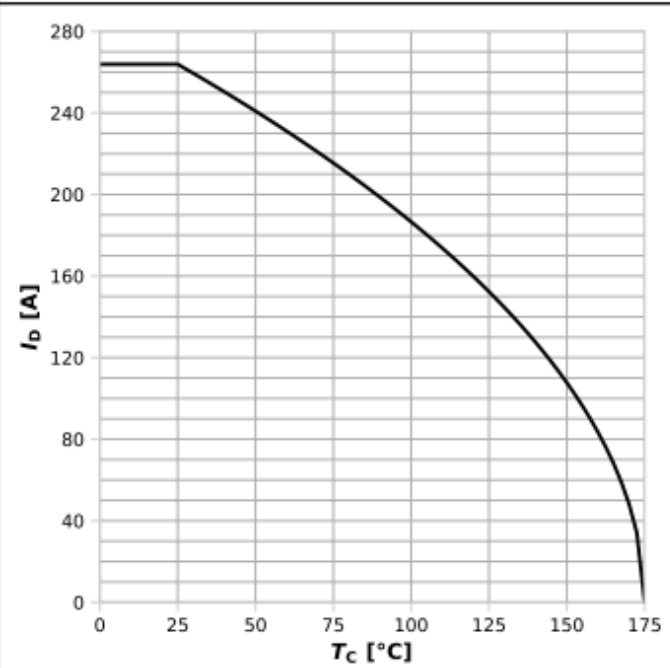
Diagram 2: Drain current
