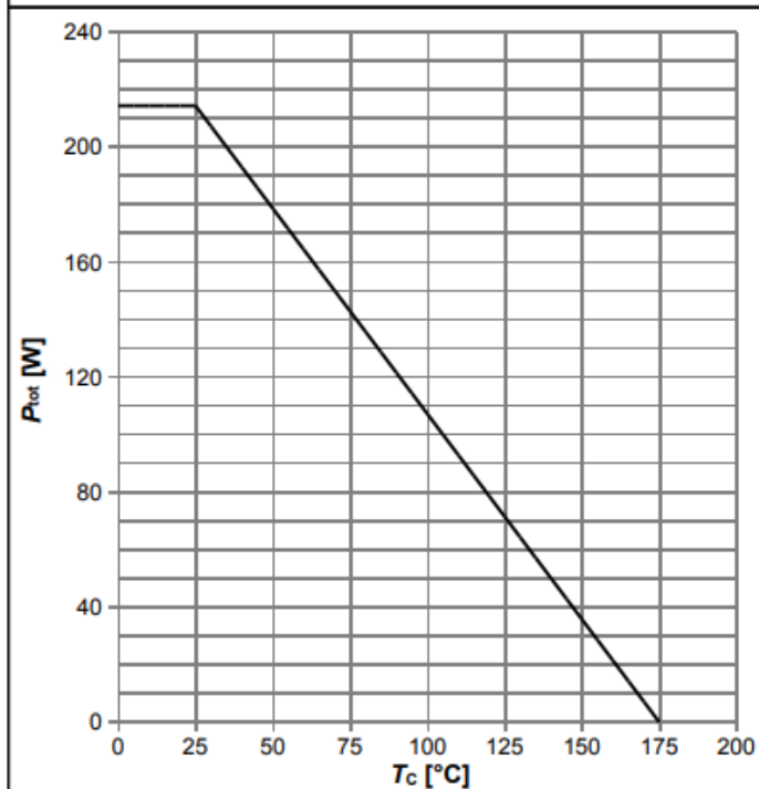
Diagram 1: Power dissipation
