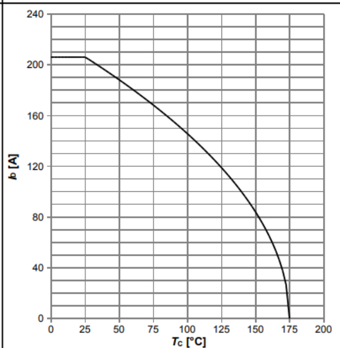
Diagram 2: Drain current
