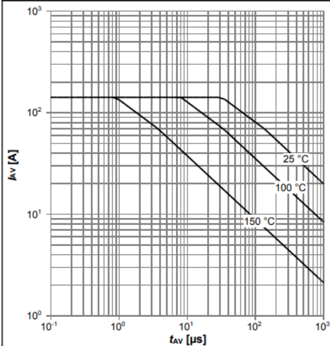
Diagram 13: Avalanche characteristics
