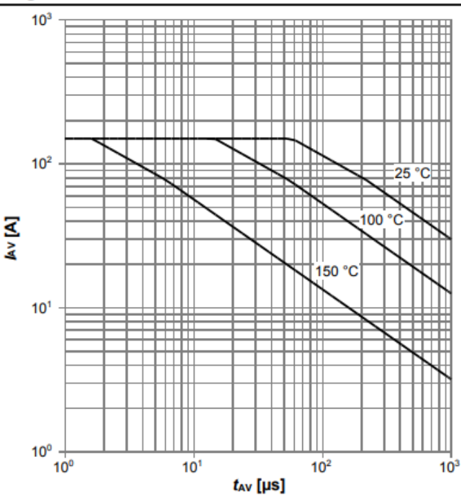
Diagram 13: Avalanche characteristics
