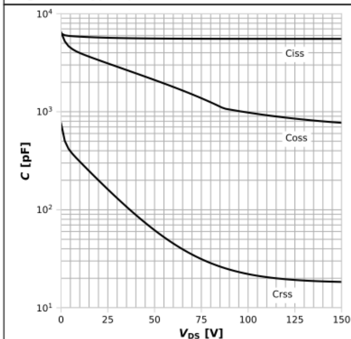
Diagram 11: Typ. capacitances
