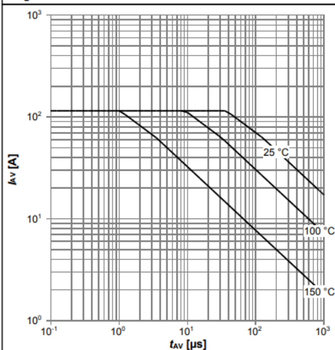
Diagram 13: Avalanche characteristics
