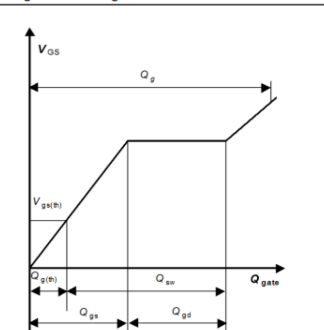
Diagram Gate charge waveforms
