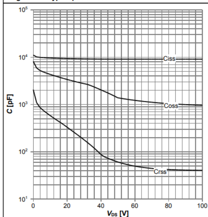
Diagram 11: Typ. capacitances
