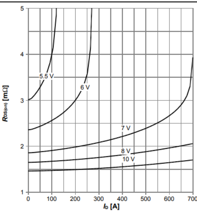
Diagram 6: Typ. drain-source on resistance
