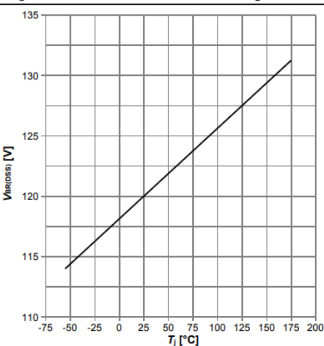
Diagram 15: Min. drain-source breakdown voltage
