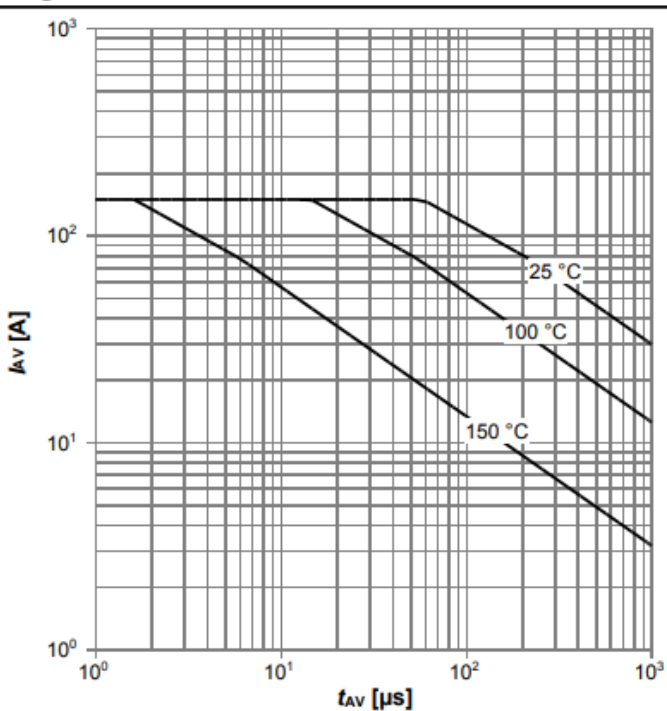
Diagram 13: Avalanche characteristics
