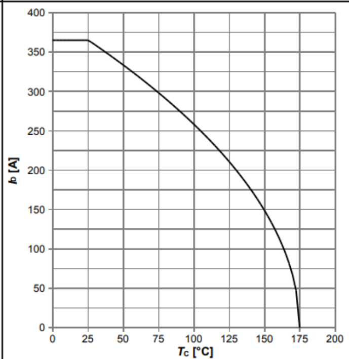
Diagram 2: Drain current
