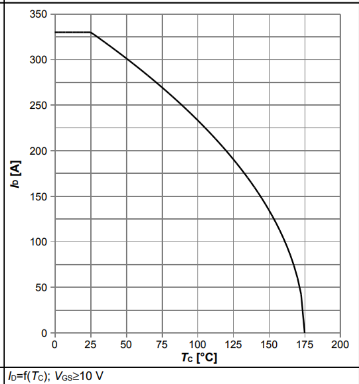
Diagram 2: Drain current
