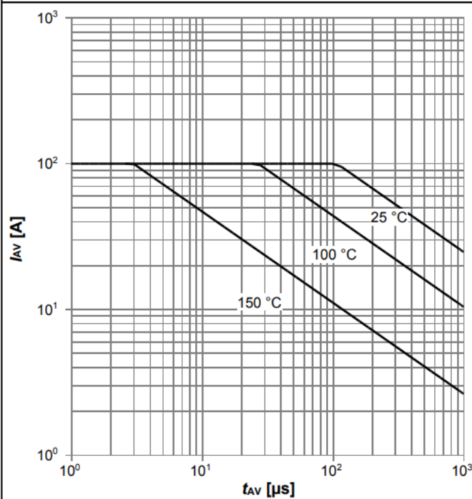
Diagram 13: Avalanche characteristics
