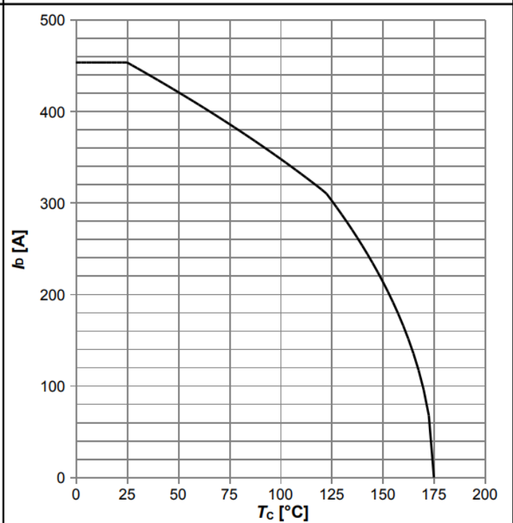
Diagram 2: Drain current
