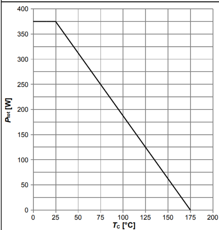
Diagram 1: Power dissipation
