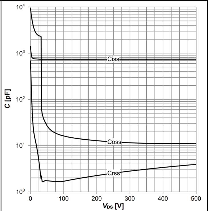
Diagram 14: Typ. capacitances
