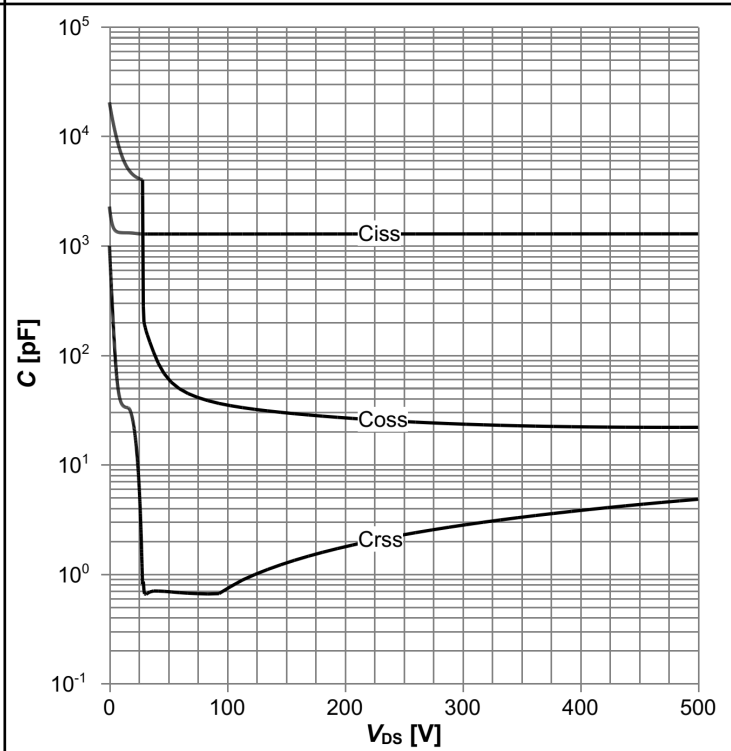
Diagram 14: Typ. capacitances
