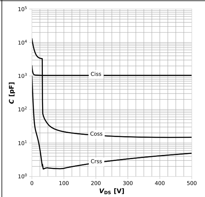
Diagram 14: Typ. capacitances
