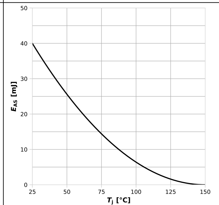
Diagram 12: Avalanche energy
