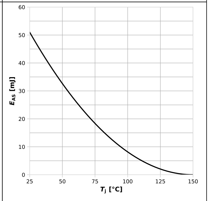
Diagram 12: Avalanche energy
