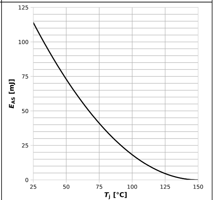
Diagram 12: Avalanche energy
