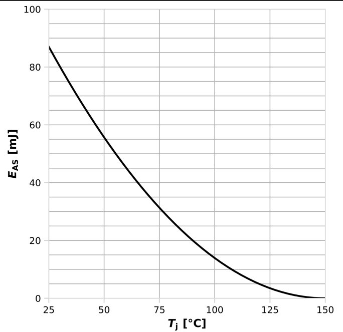
Diagram 12: Avalanche energy
