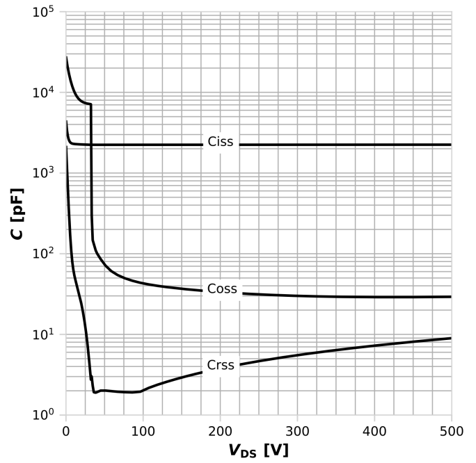
Diagram 14: Typ. capacitances
