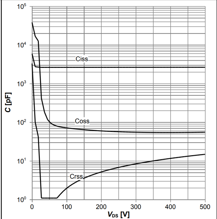
Diagram 14: Typ. capacitances
