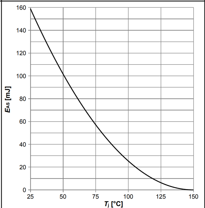
Diagram 12: Avalanche energy
