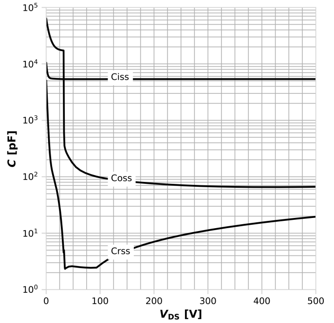
Diagram 14: Typ. capacitances
