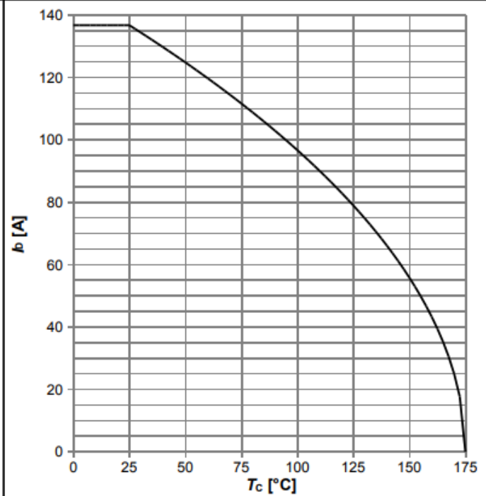
Diagram 2: Drain current
