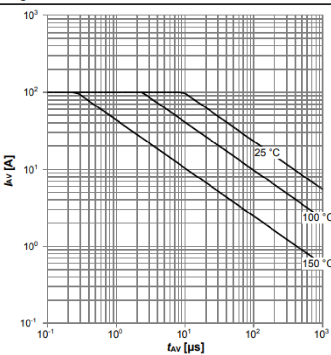
Diagram 13: Avalanche characteristics
