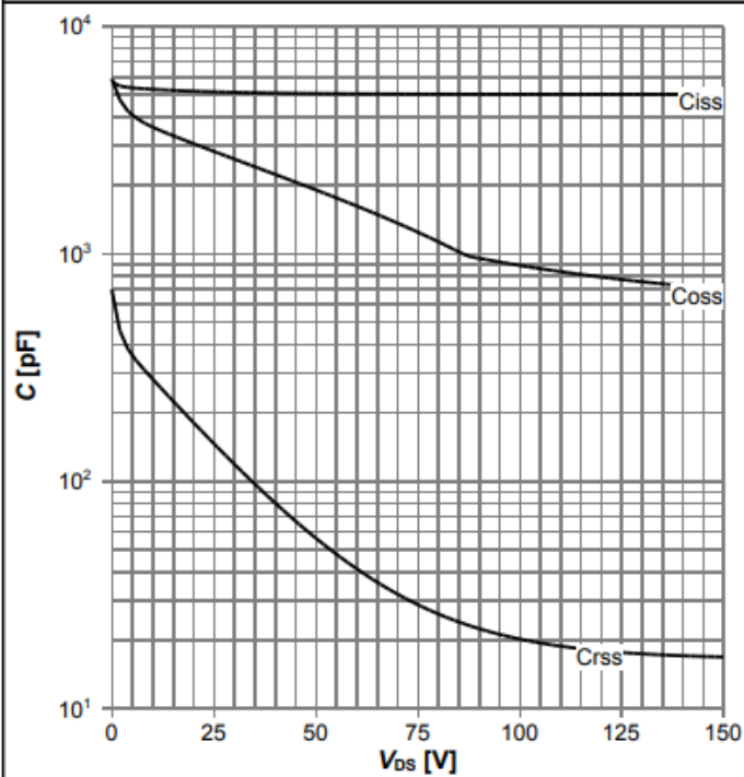
Diagram 11: Typ. capacitances
