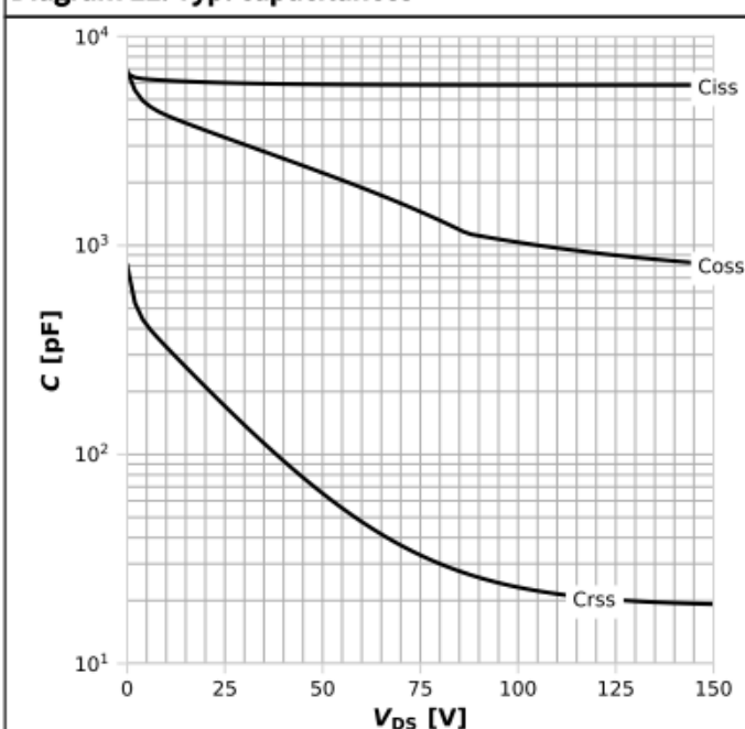
Diagram 11: Typ. capacitances
