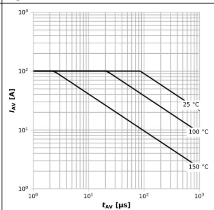
Diagram 14: Avalanche characteristics
