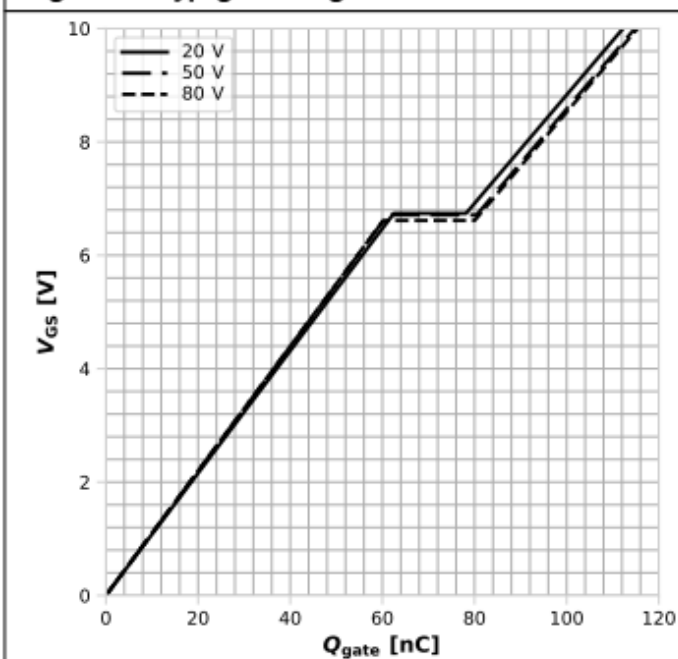
Diagram 15: Typ. gate charge
