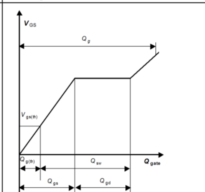
Gate charge waveforms
