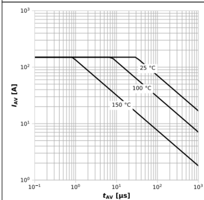
Diagram 13: Avalanche characteristics
