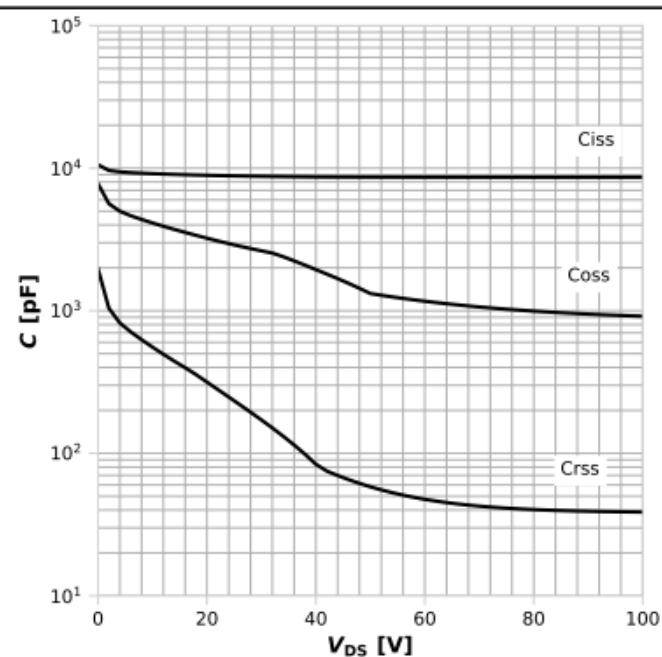
Diagram 11: Typ. capacitances
